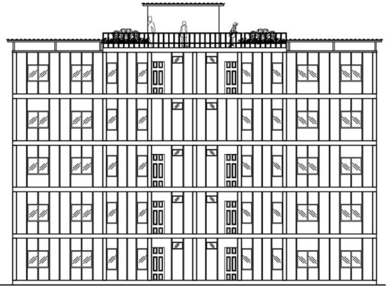
Fachada Interior E:1:125
