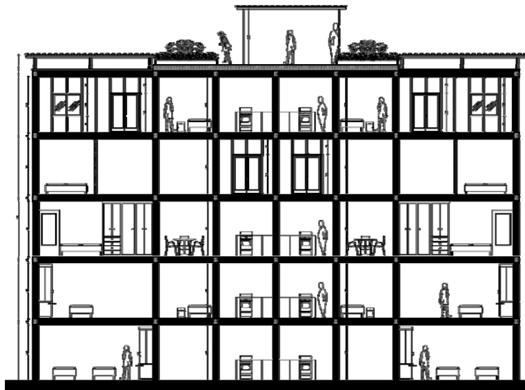
Corte B:B'' E:1:125
